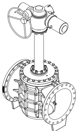
VALVE WITH EXTENDED BONNET & MOTOR OPERATOR
